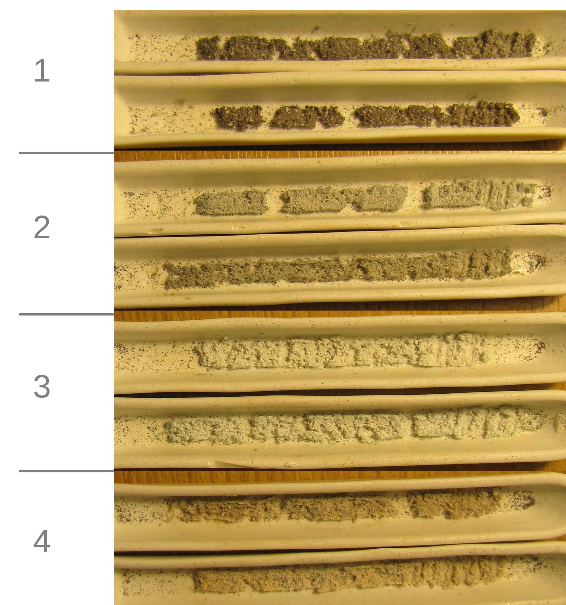
(E) Visual differences in ash melting behavior of wild plant species and Sida at 1100 °C. (1 = Common tansy; 2 = Common knapweed; 3 = Sida; 4 = Mugwort).
