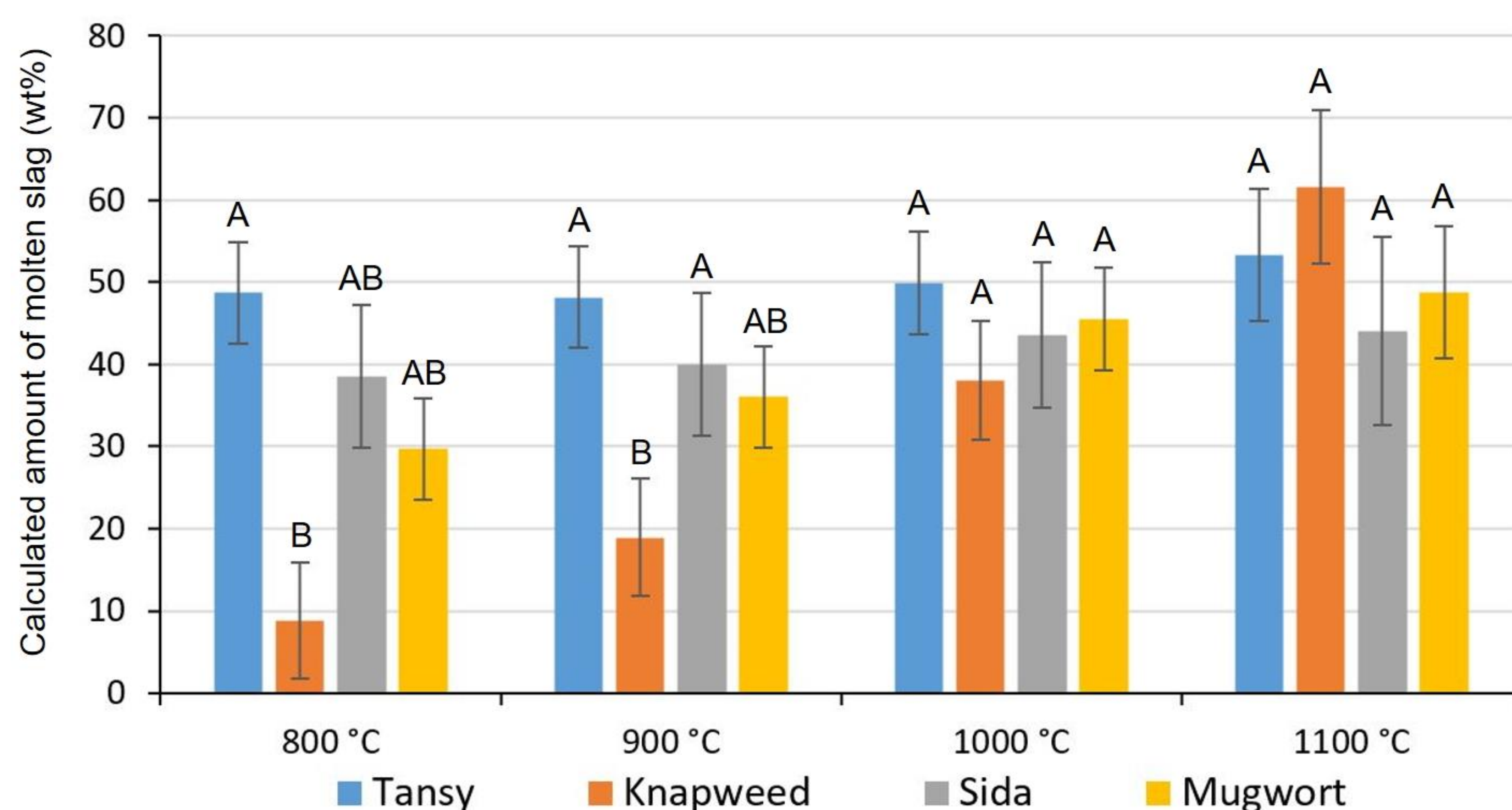
(F) Computed ash fusibility for the wild plant species and Sida. Every temperature displays the exact amount of molten slag. Different letters: significant ( p < 0.05 ) differences between crops within temperatures.
